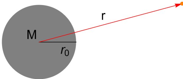
Figure: We consider the Schwarzschild-de Sitter metric of nonlocal \sqrt{dS} gravity at the distances far from a spherically symmetric massive body.
