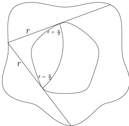
Рис.: Magnetic billiard with Gutkin property for \delta = \pi/2 .
