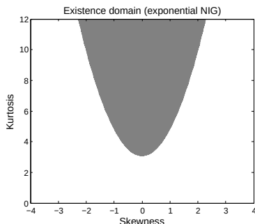
Figure : Existence domain for the moment calibration problem (2) under the VG and Meixner exponential models (left) and under the NIG exponential model (right).
