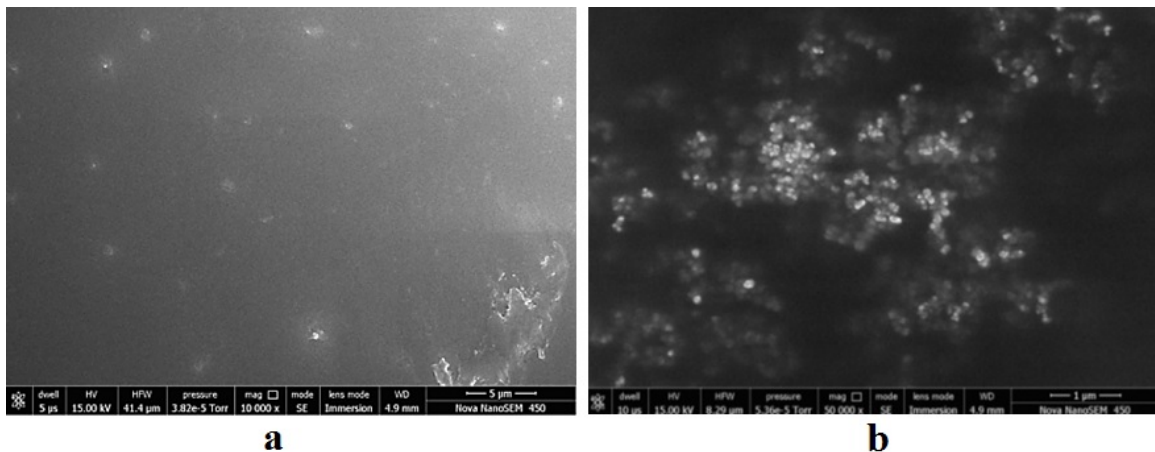
FIG. 2. SEM images of (a) \text{Bi}_2\text{Te}_{2.7}\text{Se}_{0.3} (b) \text{Sb}_2\text{Te}_3
